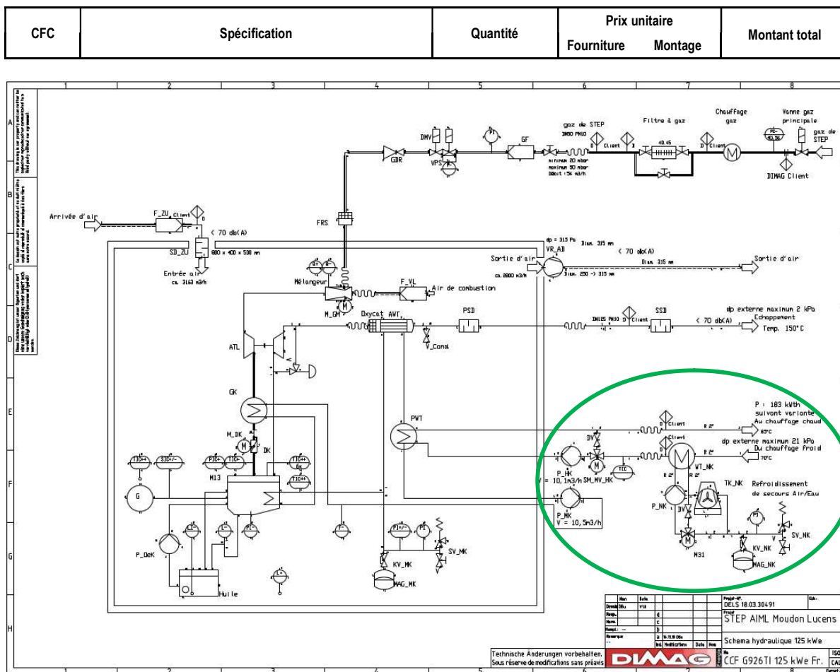
Figure 1 : Illustration des limites de fourniture CCF I & CCF II (Source Techfina SA)
