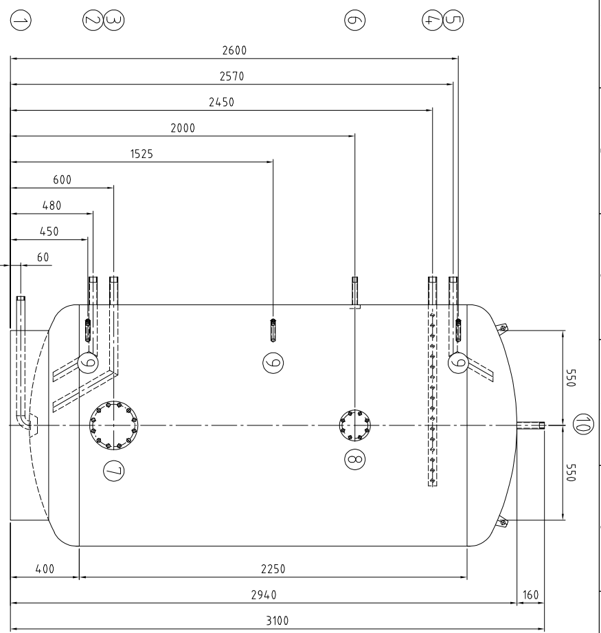
Detail Pos. 2.5 / detail pos.2.5
