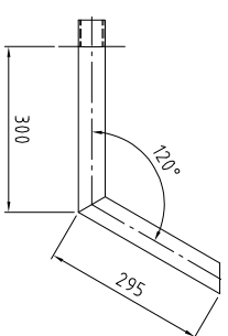
Detail Pos. 2.5 / detail pos.2.5
